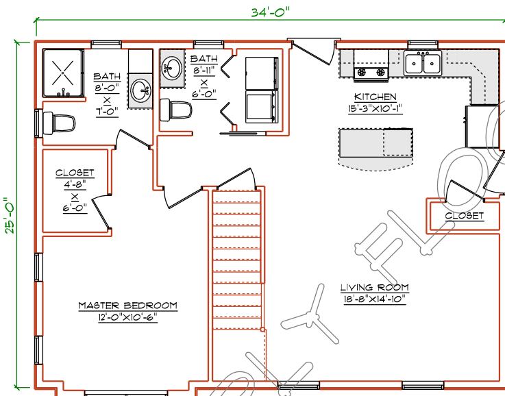
LEVEL ONE PLAN
