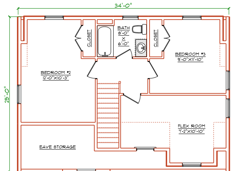
LEVEL TWO PLAN
