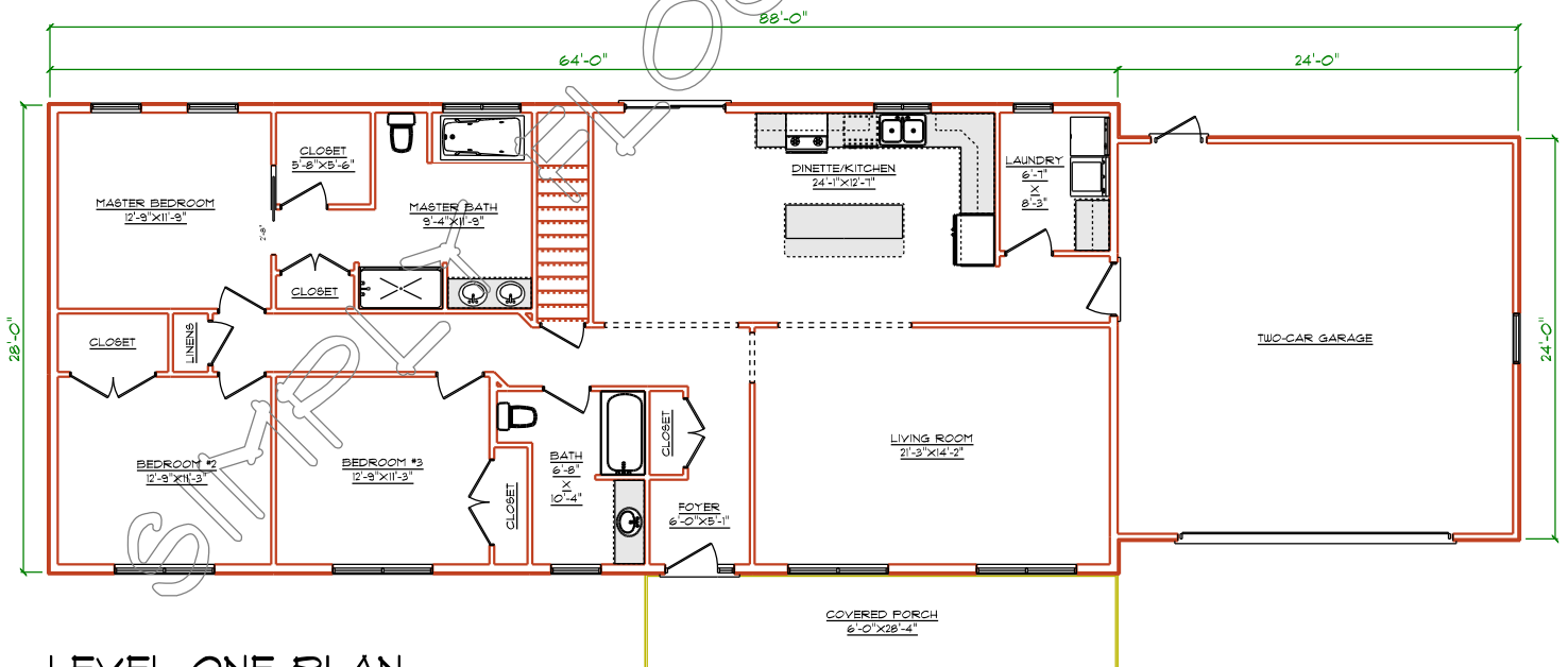
LEVEL ONE PLAN
