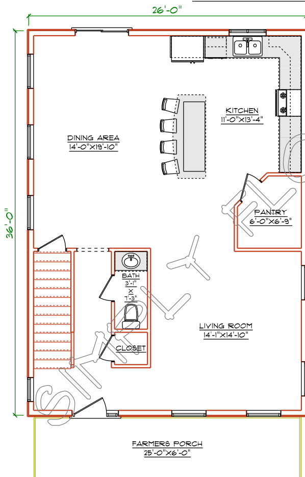
LEVEL ONE PLAN
