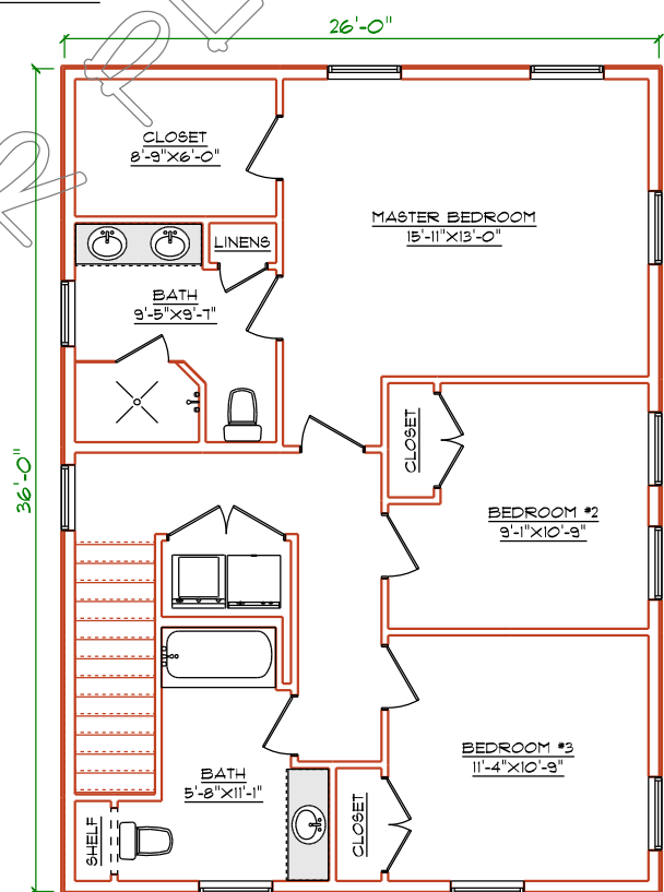
LEVEL TWO PLAN
