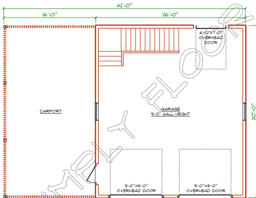
LEVEL ONE PLAN
