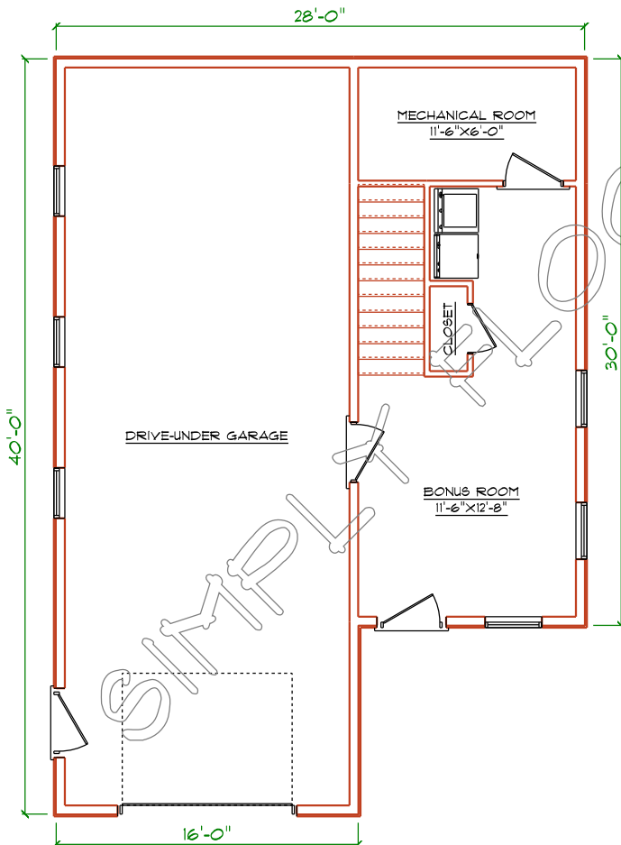
LEVEL ONE PLAN
