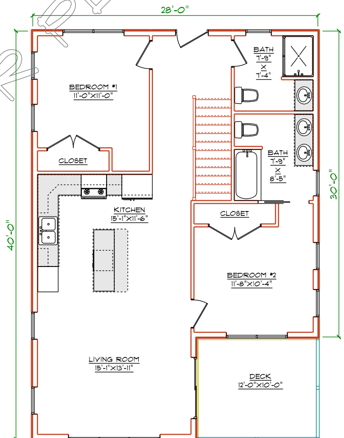
LEVEL TWO PLAN
