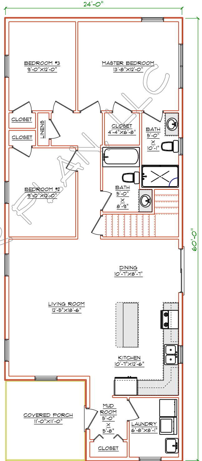
LEVEL ONE PLAN
