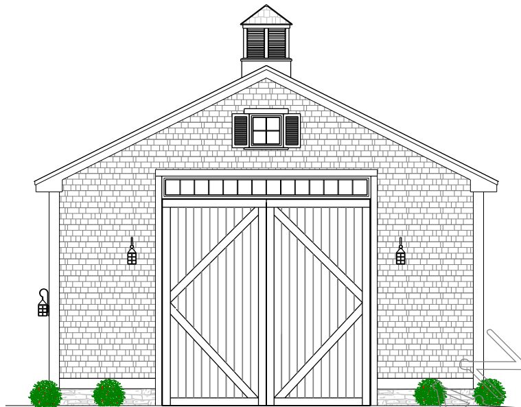
FRONT ELEVATION
