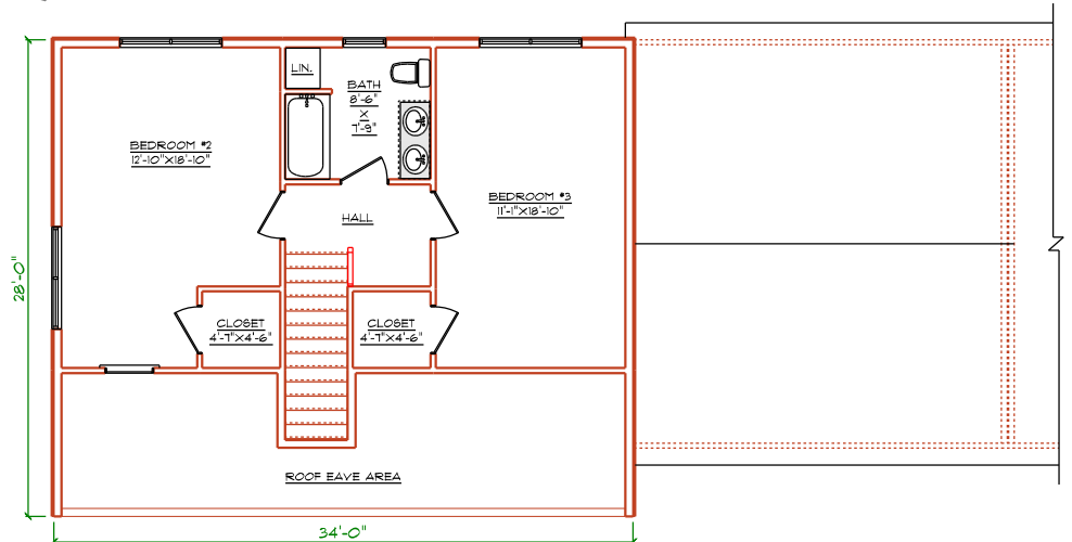
LEVEL TWO PLAN
