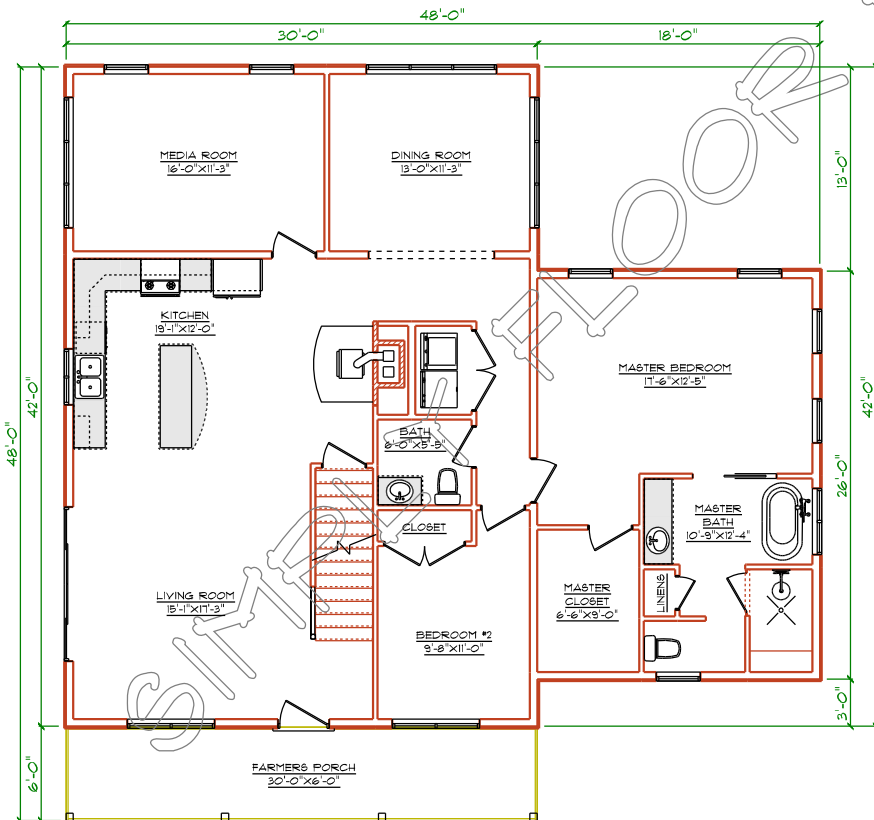
LEVEL ONE PLAN
