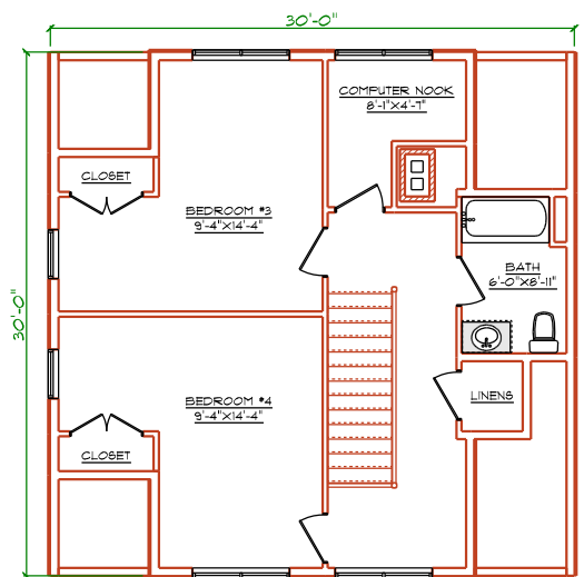
LEVEL TWO PLAN
