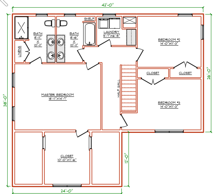
LEVEL TWO PLAN
