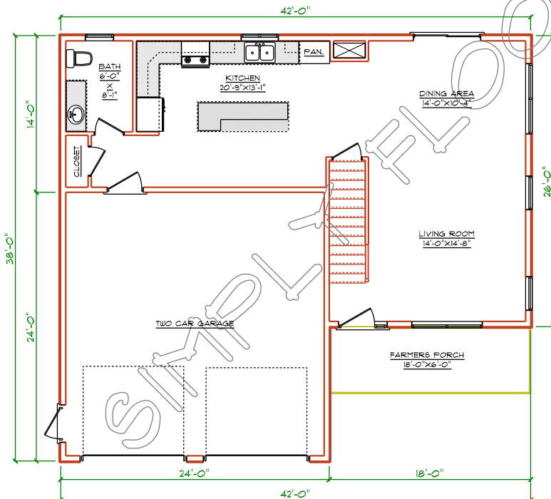
LEVEL ONE PLAN
