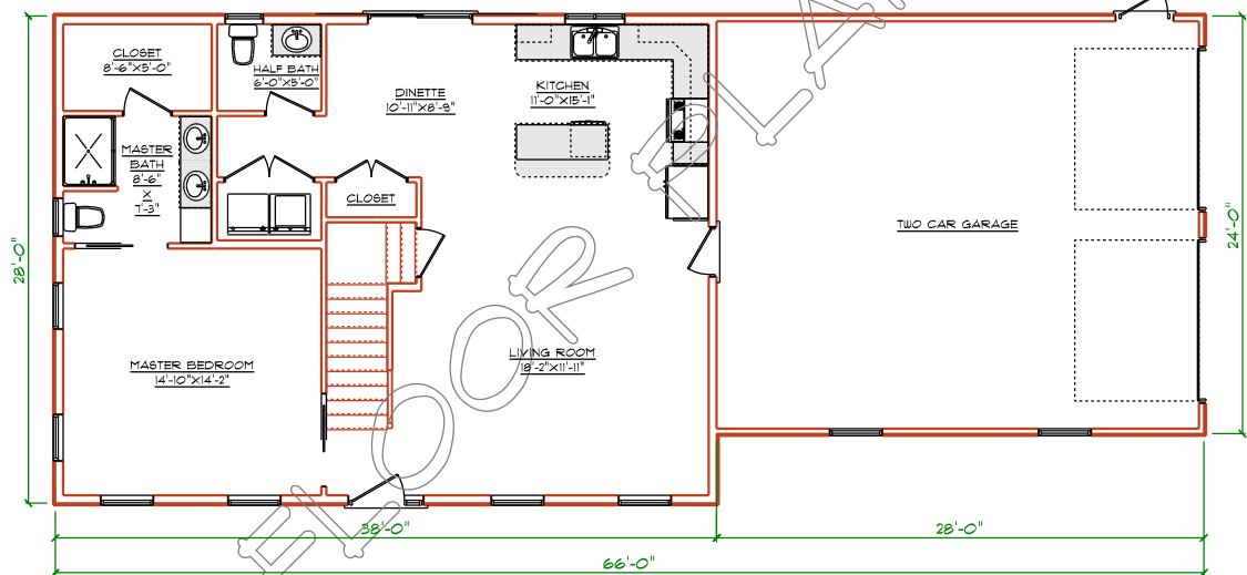
LEVEL ONE PLAN
