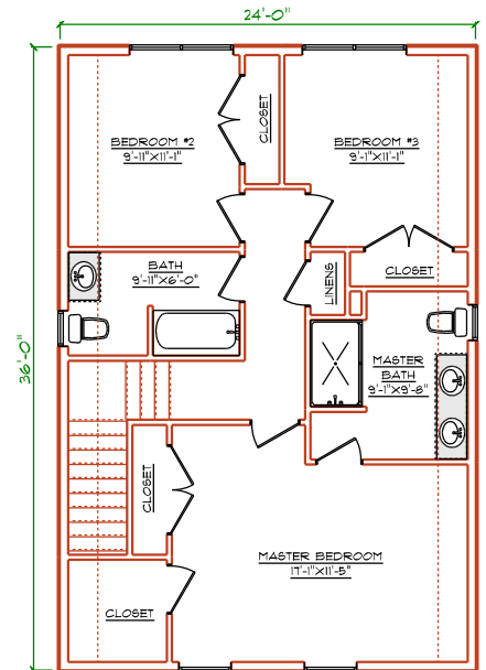
LEVEL TWO PLAN
