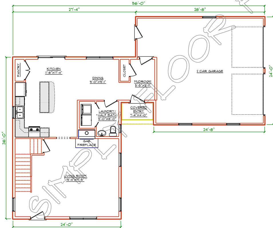
LEVEL ONE PLAN
