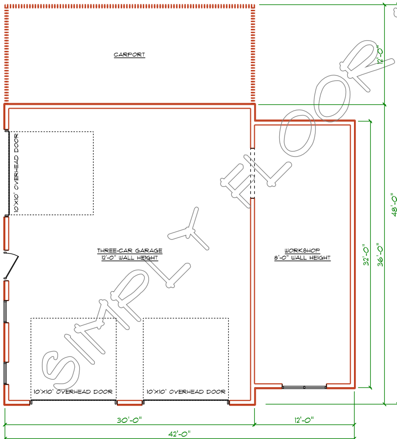
LEVEL ONE PLAN
