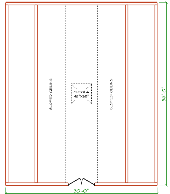
LEVEL TWO PLAN
