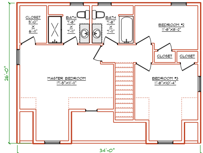
LEVEL TWO PLAN
