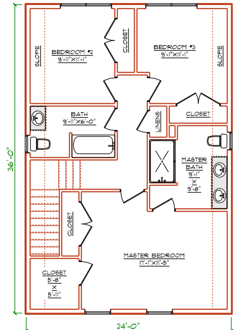
LEVEL TWO PLAN
