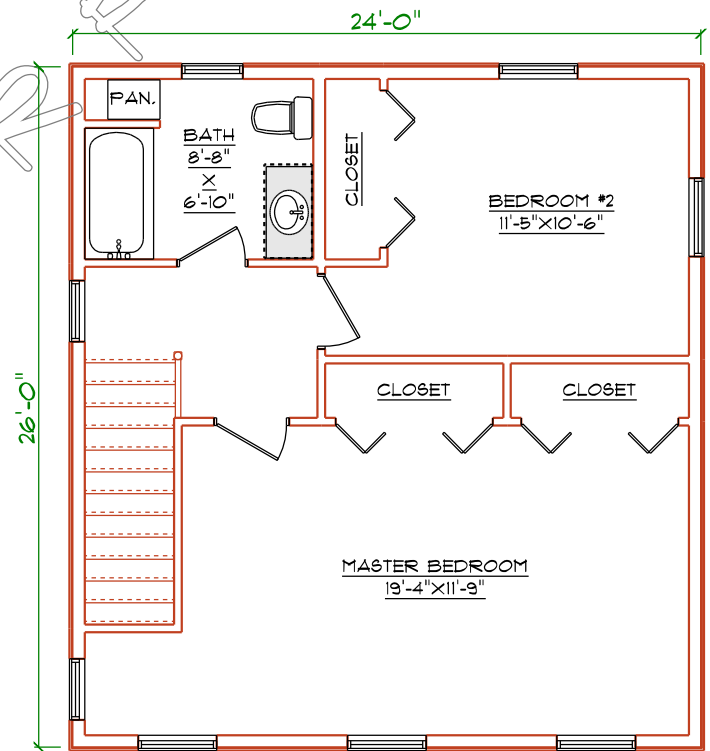
LEVEL TWO PLAN
