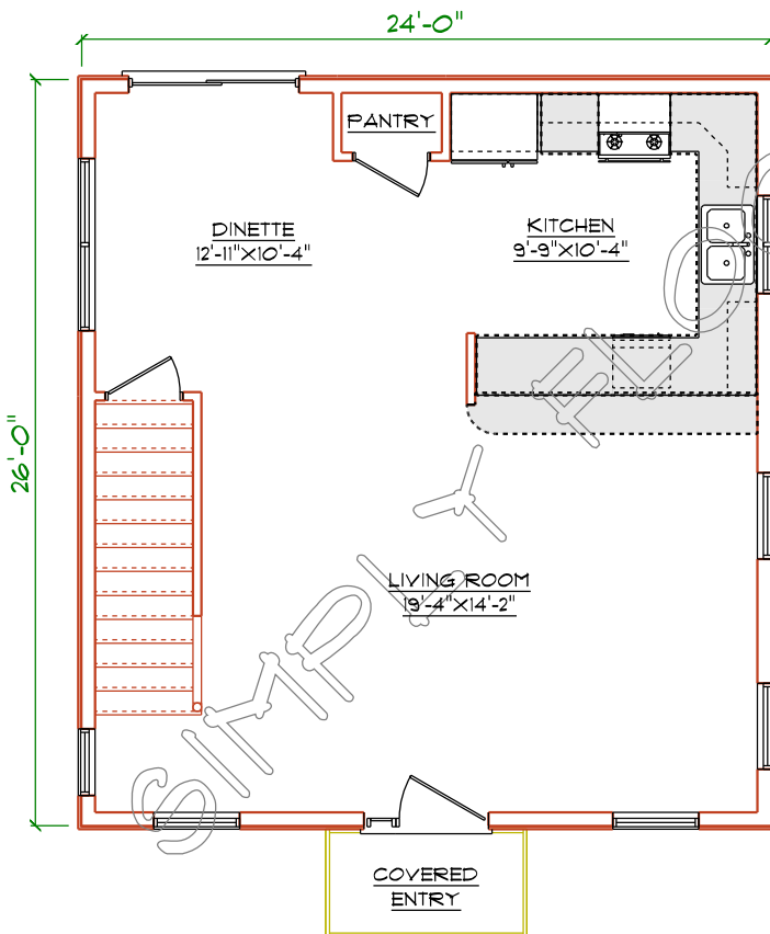
LEVEL ONE PLAN
