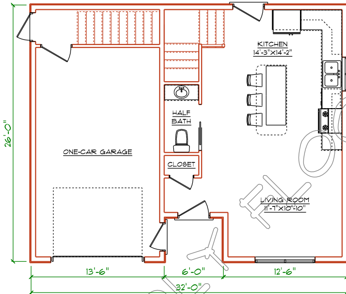
LEVEL ONE PLAN
