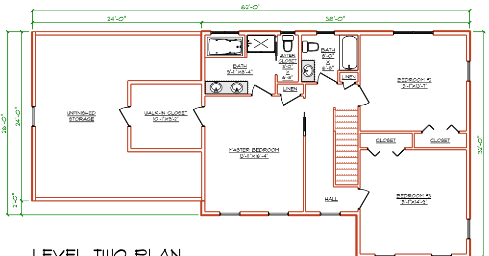
LEVEL TWO PLAN
