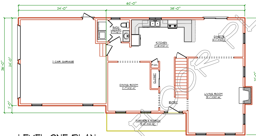
LEVEL ONE PLAN
