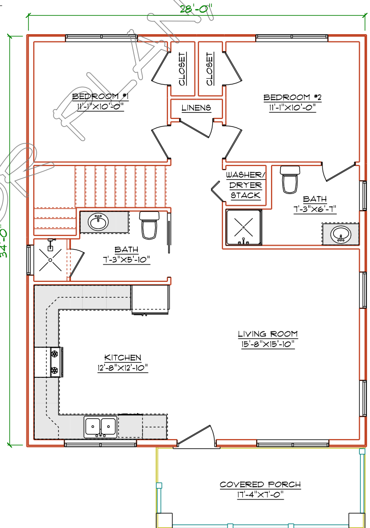
LEVEL TWO PLAN
