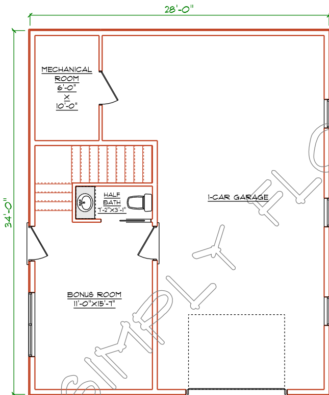
LEVEL ONE PLAN
