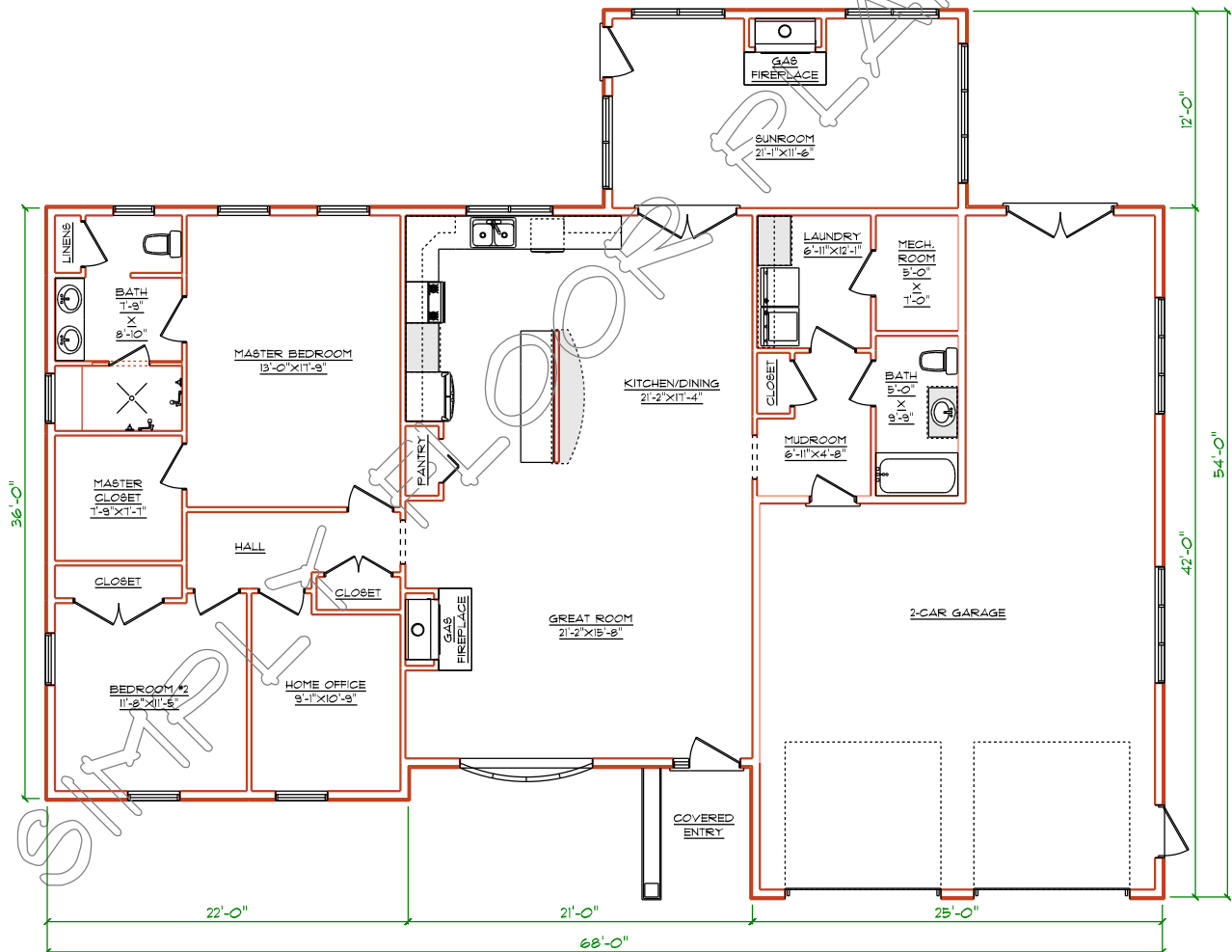
LEVEL ONE PLAN
