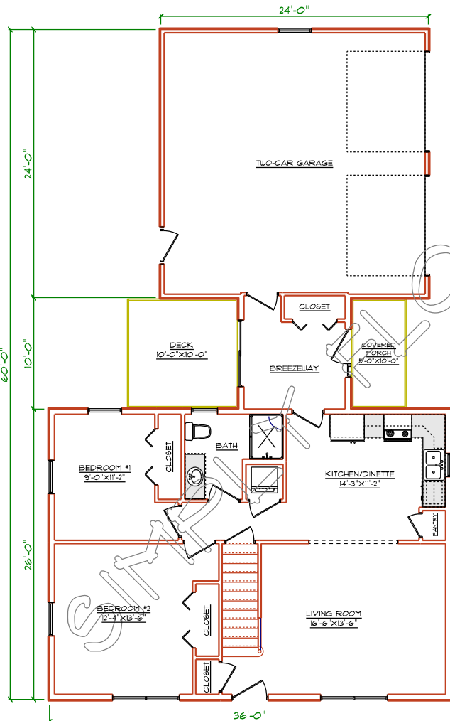
LEVEL ONE PLAN
