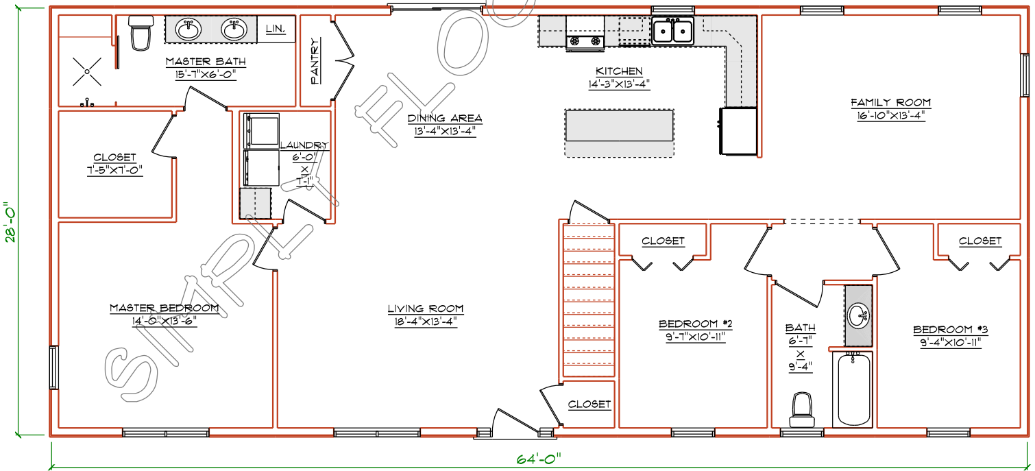
LEVEL ONE PLAN
