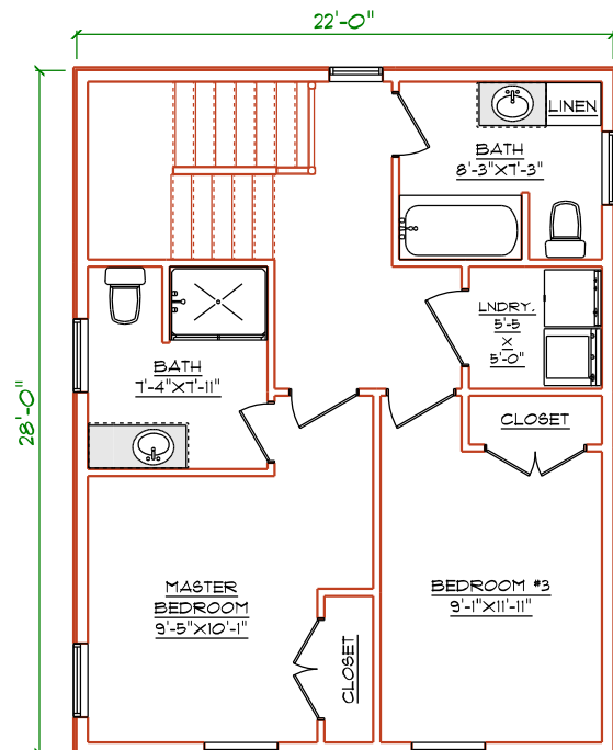
LEVEL THREE PLAN
