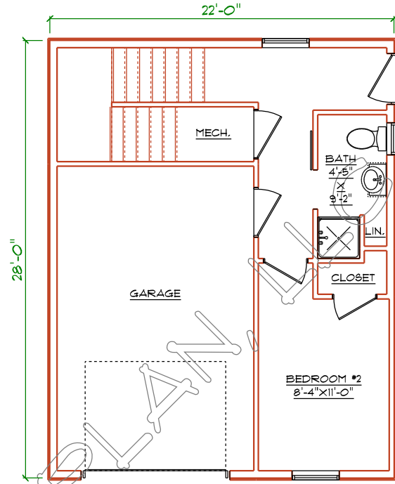
LEVEL ONE PLAN
