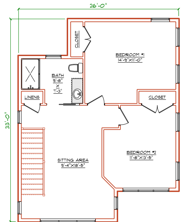
LEVEL TWO PLAN
