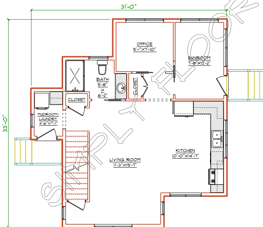
LEVEL ONE PLAN
