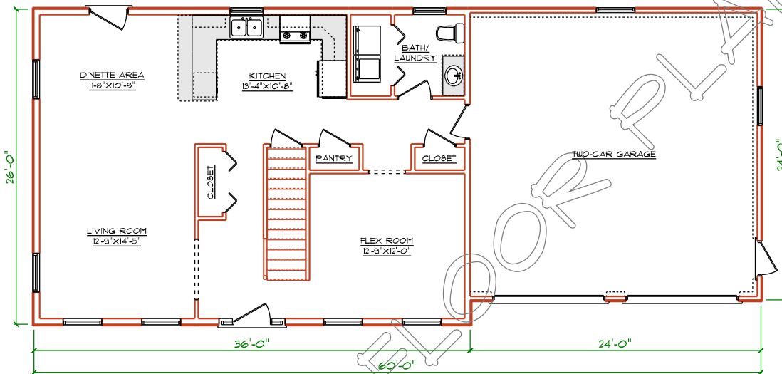
LEVEL ONE PLAN
