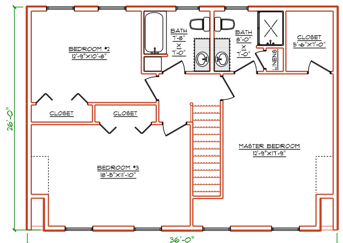
LEVEL TWO PLAN
