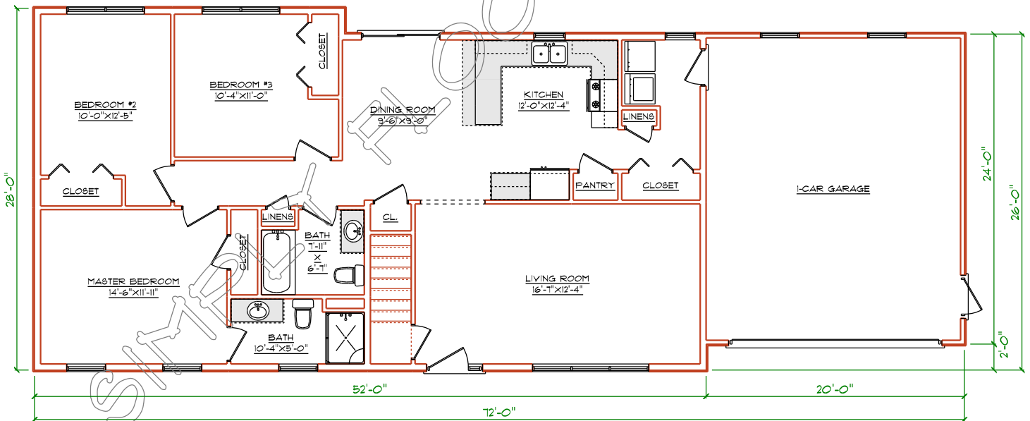
LEVEL ONE PLAN
