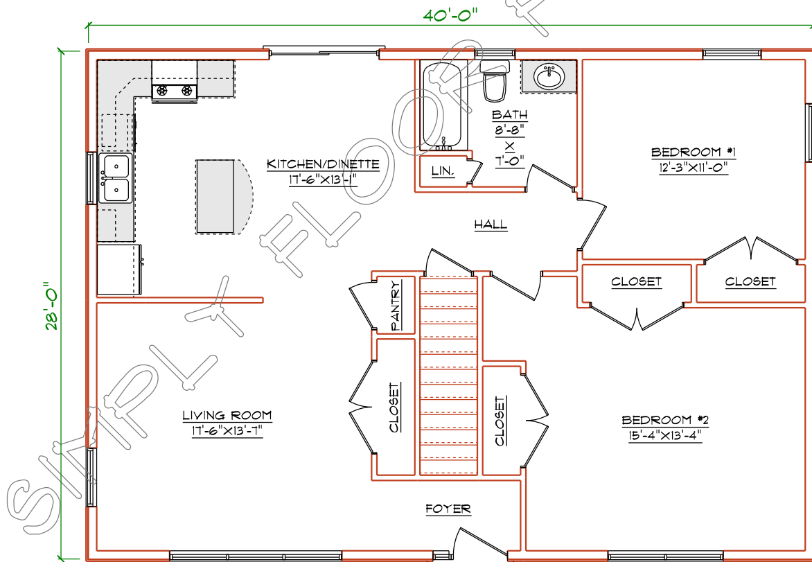
LEVEL ONE PLAN
