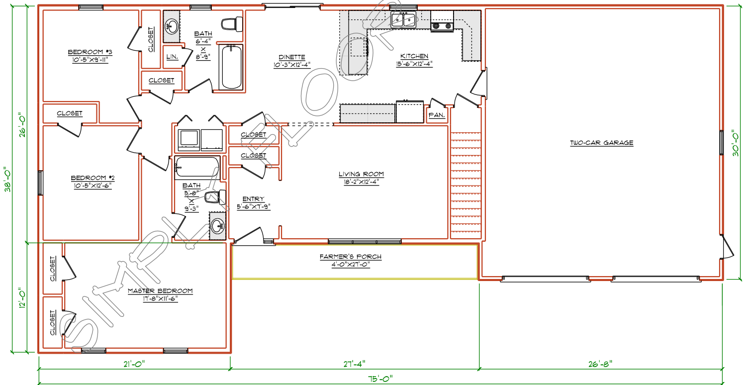
LEVEL ONE PLAN
