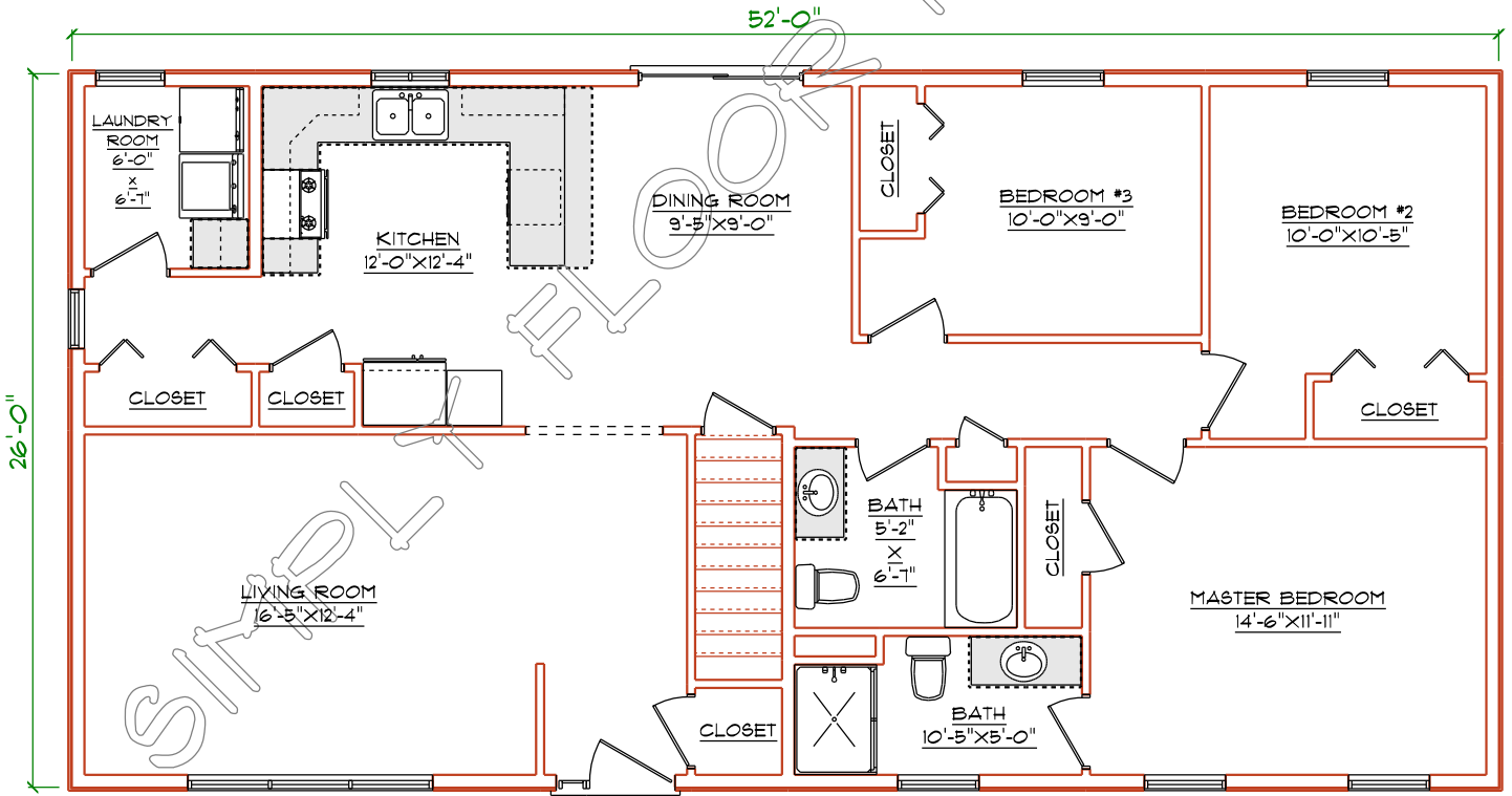
LEVEL ONE PLAN
