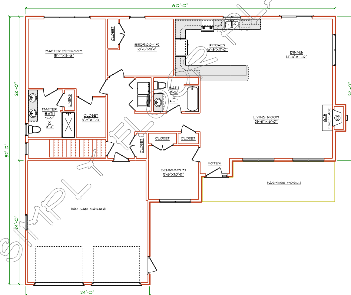
LEVEL ONE PLAN
