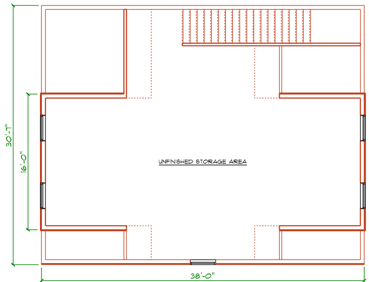
LEVEL TWO PLAN
