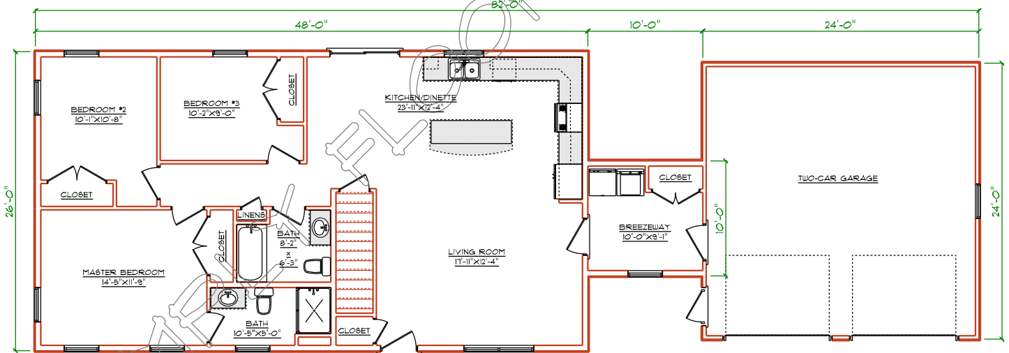
LEVEL ONE PLAN
