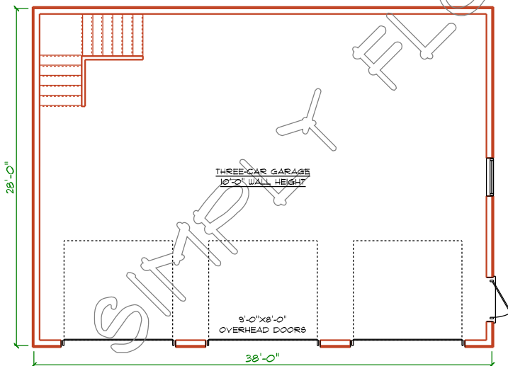
LEVEL ONE PLAN
