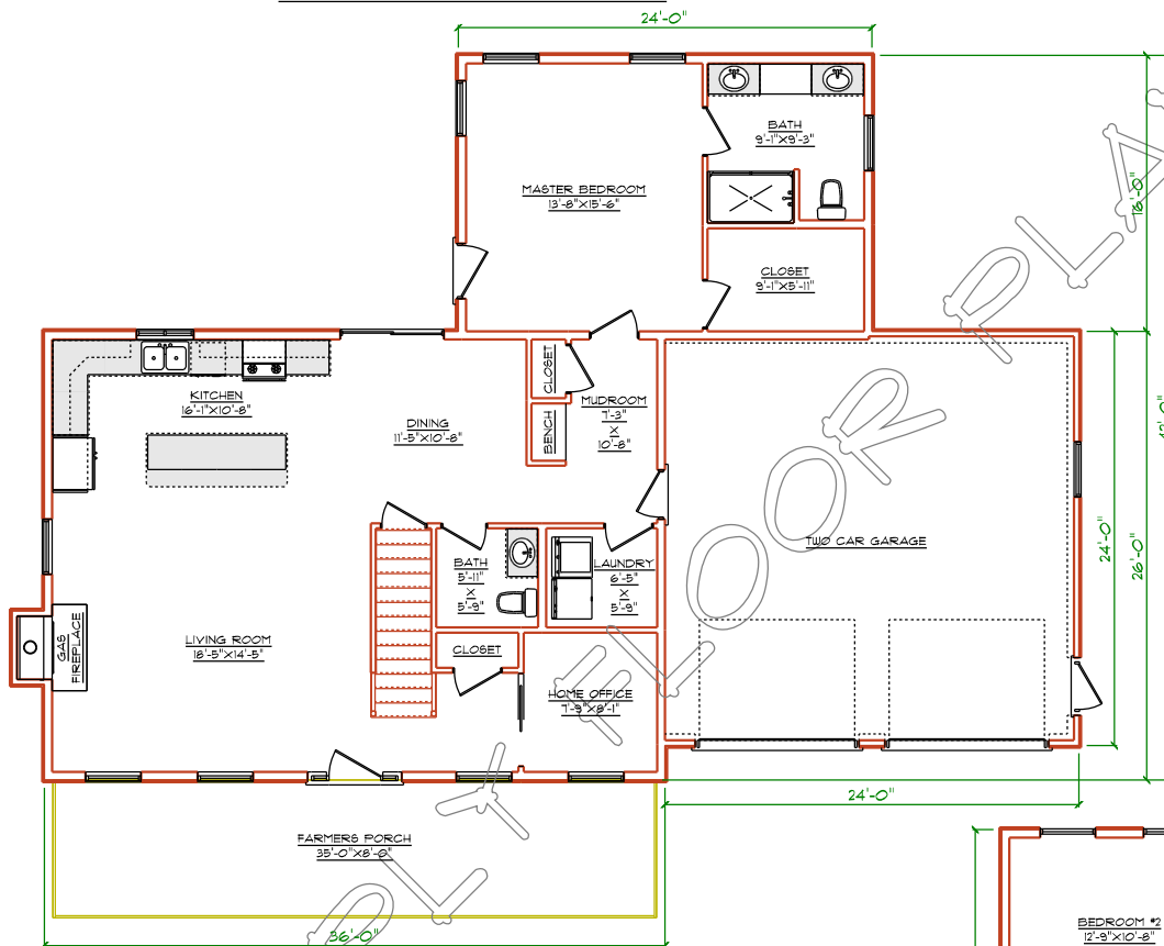
LEVEL ONE PLAN
