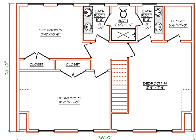
LEVEL TWO PLAN
