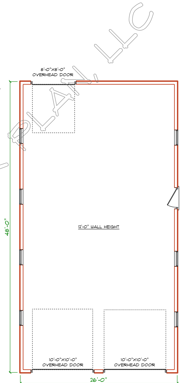
GARAGE FLOOR PLAN
