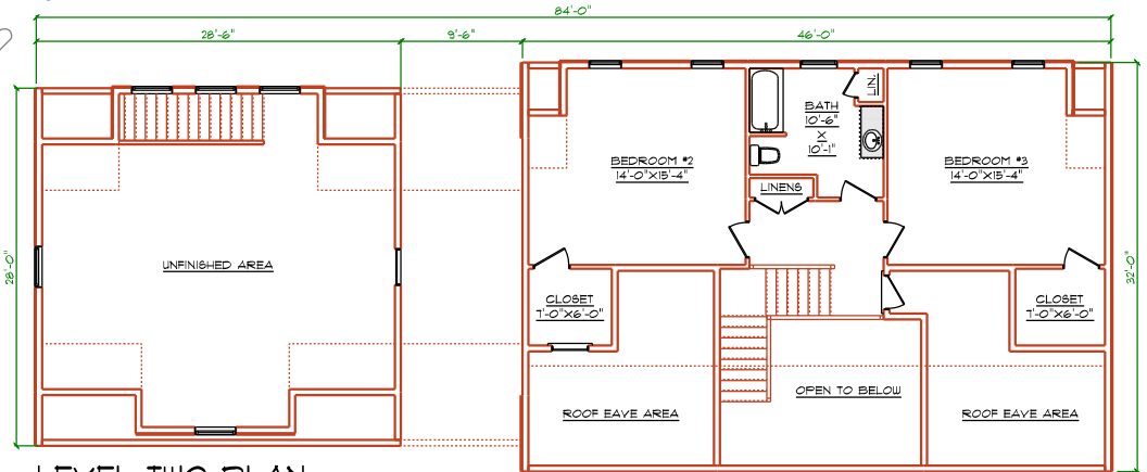
LEVEL TWO PLAN 785 +/- SQUARE FEET
