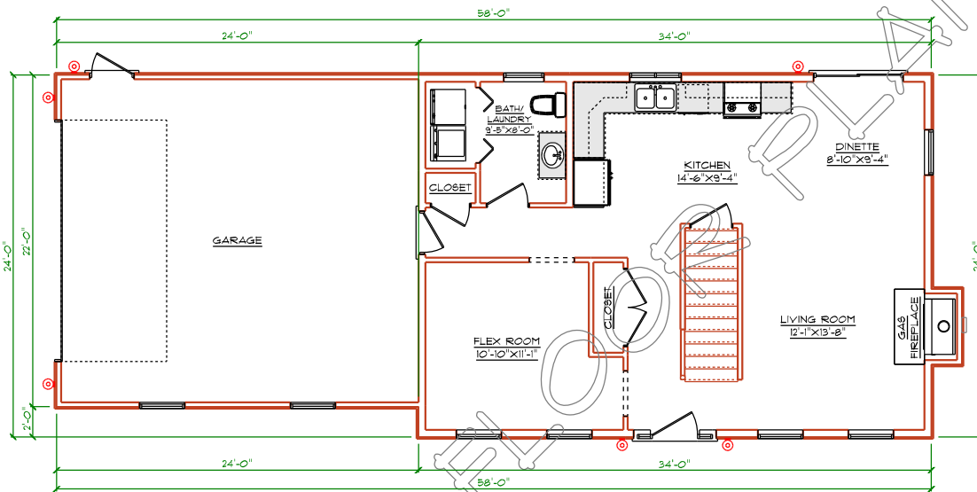
LEVEL ONE PLAN
