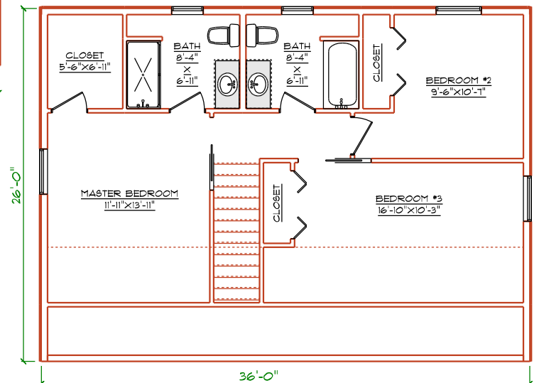
LEVEL TWO PLAN
